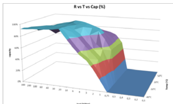
Graph 11: Capacity de-rating plot of an ER-1/2AA cell
