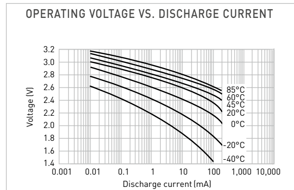
Graph 8: Operating voltage of a Panasonic BR-2/3A cell
